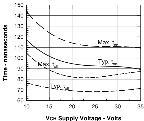
Fig. 13b. High side turn-on and turn-off delay times vs. V_{CH} .
