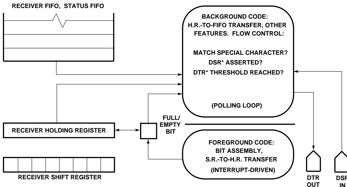
Figure 5-5. Receiver Flow-Control Logic
