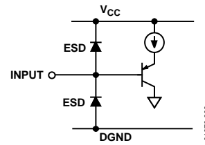
Figure 46. Logic Input
