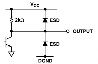
Figure 47. Logic Output
