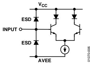
Figure 43. Analog Input
