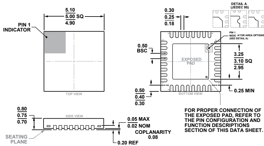
COMPLIANT TO JEDEC STANDARDS MO-220-WHHD Figure 28. 32-Lead Lead Frame Chip Scale Package [LFCSP] 5 mm × 5 mm Body and 0.75 mm Package Height (CP-32-7) Dimensions shown in millimeters
