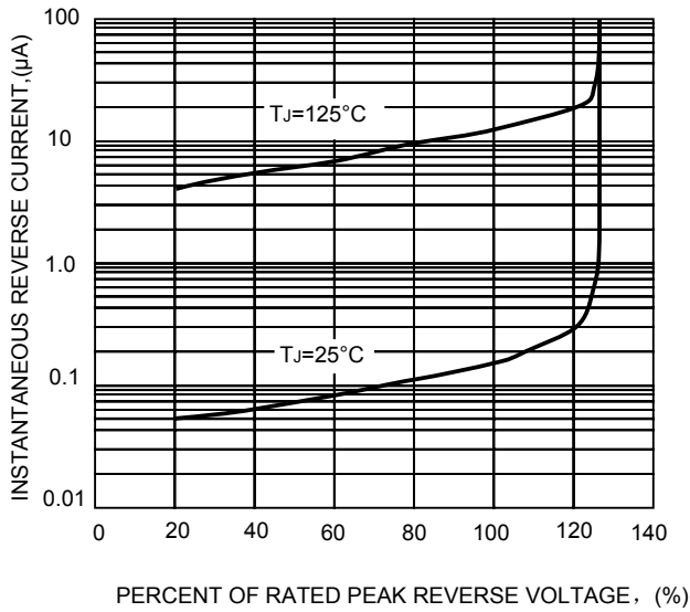
FIG.3-TYPICAL REVERSE CHARACTERISTICS
